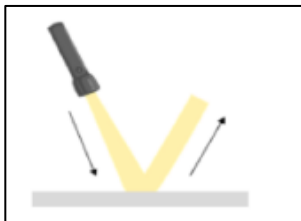
Left: Light travelling and reflecting off a smooth surface
